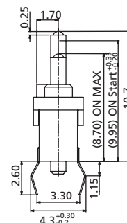
DF1HHA High Actuator
