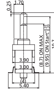
DF1SHA High Actuator
