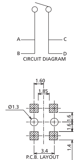
DF1SHA High Actuator
