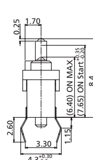
DF1HNA Standard Actuator
